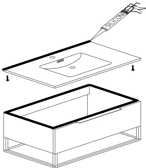
Silicone Sealant
