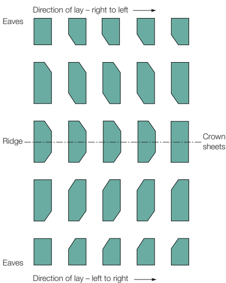
Fig. 3 Mitring plan - double slope roof
