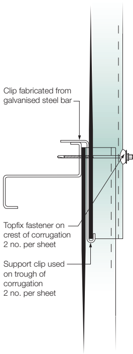
Fig.1 - Single skin vertical profiled sheeting
