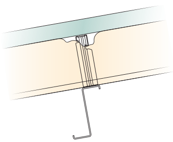
Fig.1 - Steel liner, spacer bar system, quilt insulation
