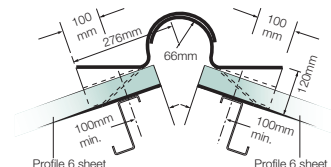
Fig.3 - Two piece ventilating ridge
