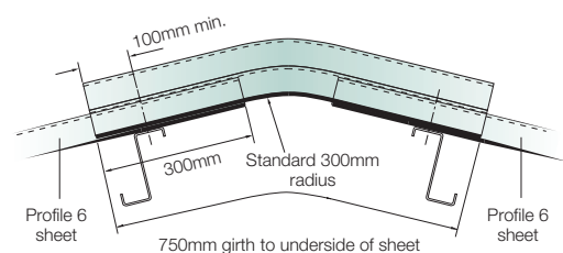
Fig.2 - Ventilating cranked crown fixings
