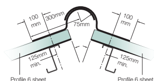
Fig.2 - Two piece plain wing ridge
