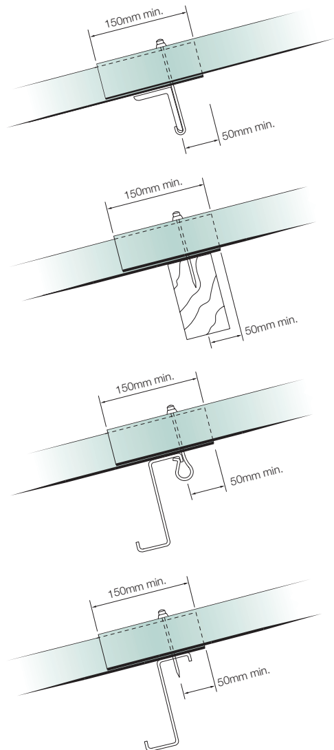
Fig. 5 Typical fixing details
