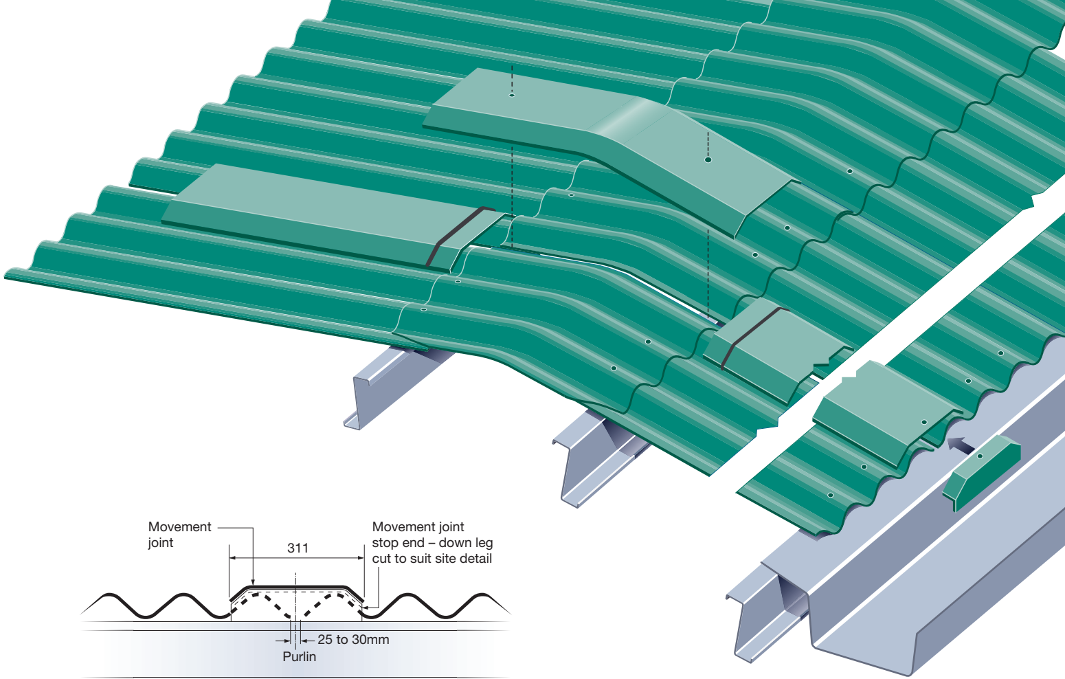
Fig.1 - Movement joint end elevation
