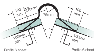
Fig.1 - Two piece close fitting ridge
