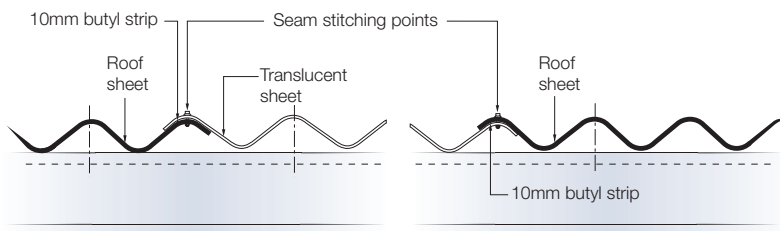
Fig.2 - Side lap detail for translucent sheet rooflights
