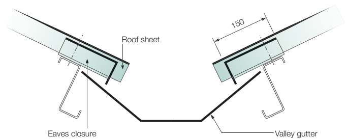
Fig.1 - valley gutter fixings
