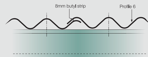
Fig.1a Profile 6 side lap
