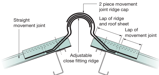
Fig.3 - Movement joint ridge cap
