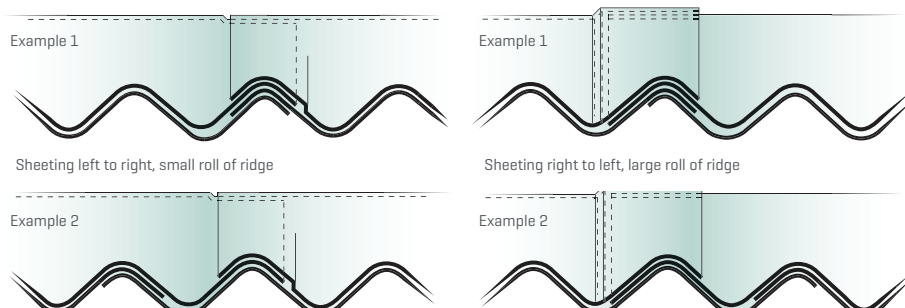
Fig.4 - Position of two piece ridges
