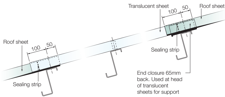
Fig.1 - End lap details for translucent sheet rooflights
