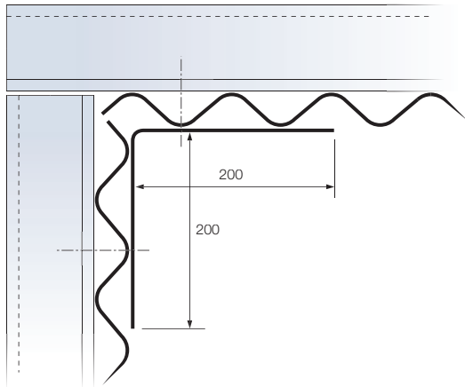
Fig.3 - Internal corner section
