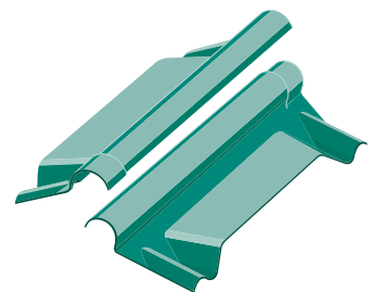
Fig.6 Two piece ventilating ridge piece
