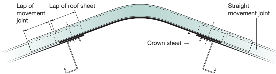
Fig.2 - Movement joint side elevations
