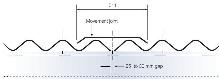
Fig.4 - Vertical movement joint
