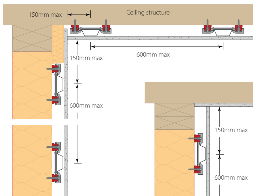
Resiliently mounted ceiling
