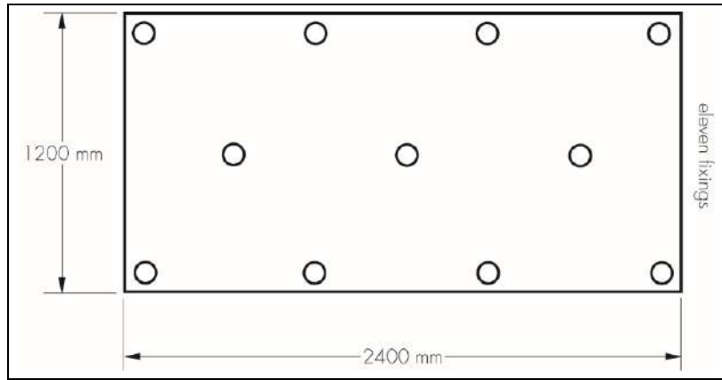
Figure 1 Fastener layout
