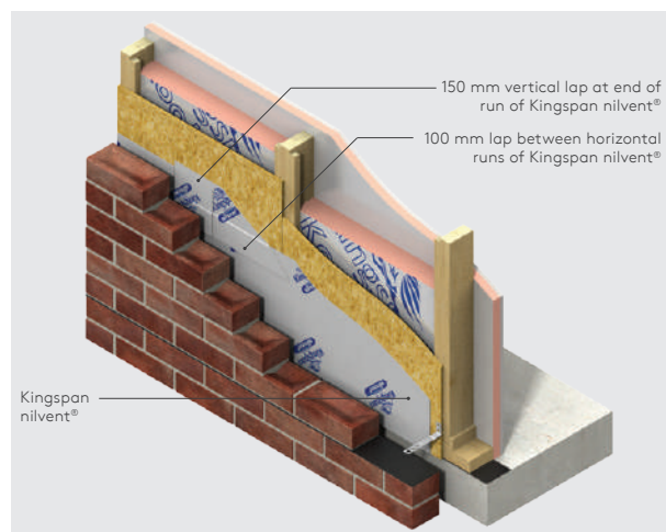
Figure 4 - External masonry
