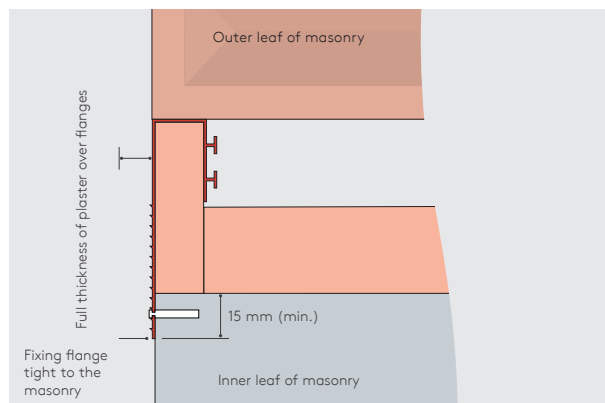
Figure 12: Basic installation principles
