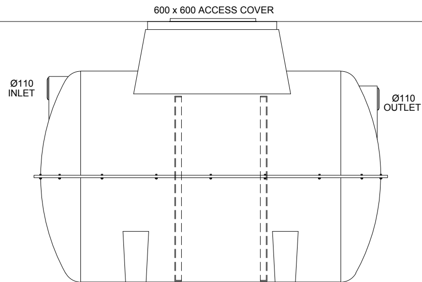
SIDE ELEVATION
