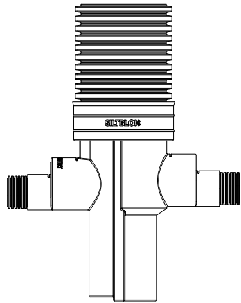
Ø 150 PIPEWORK
