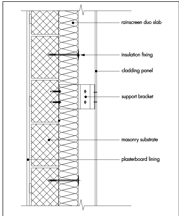
Figure 3 Masonry substrate
