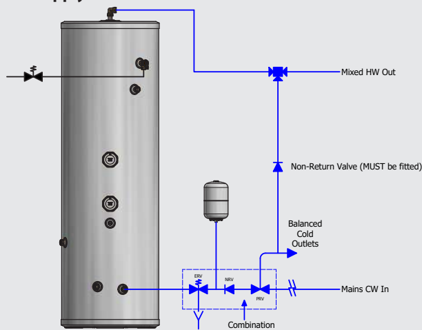
Figure 2: Cold port of the blending valve connected to balanced cold supply - NON-RETURN VALVE MUST BE FITTED
