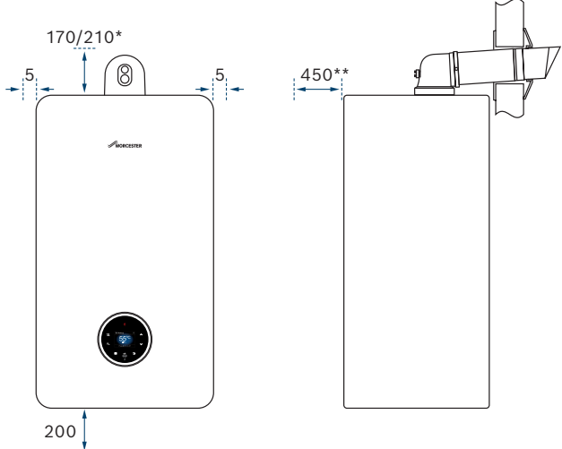
Clearances (mm)
