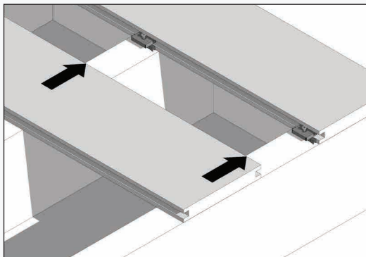
⑤ Slide and tap the next board in place
