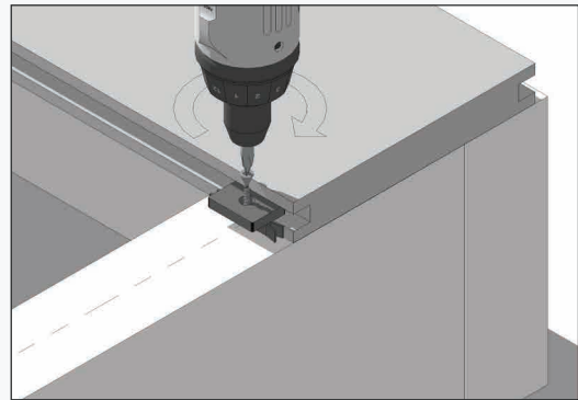
④ Screw down lightly to the deck bearer
