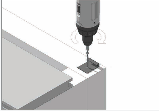
① Fix starter clips to the outer edge of your deck
