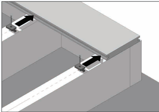
③ Place the hidden fasteners into the board edge
