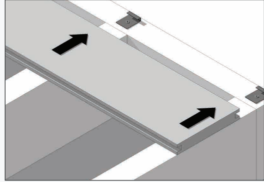
② Slide the first board into the starter fasteners
