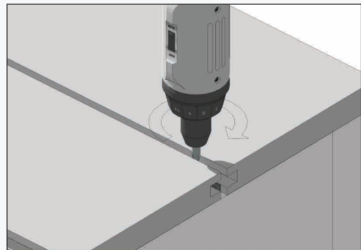
⑥ Tighten the hidden fasteners to secure the board
