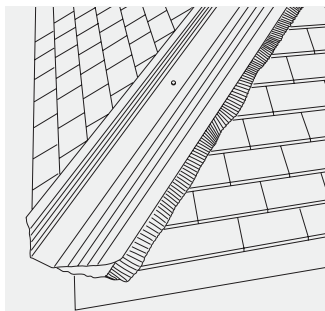
Fig. 60 – HipFast support tray cut at eaves
