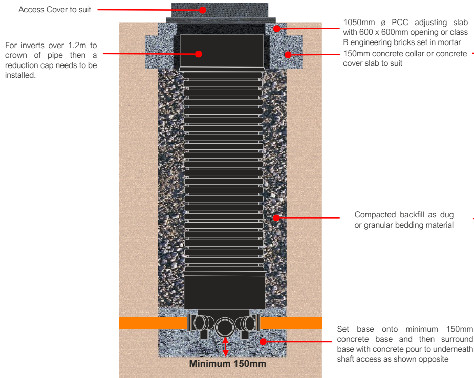
Typical installation for IC110 &160 kits with base
