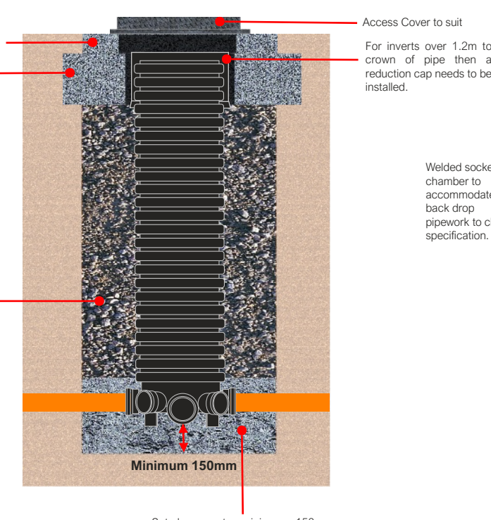
Typical installation for IC110 & 160 SP single piece units
