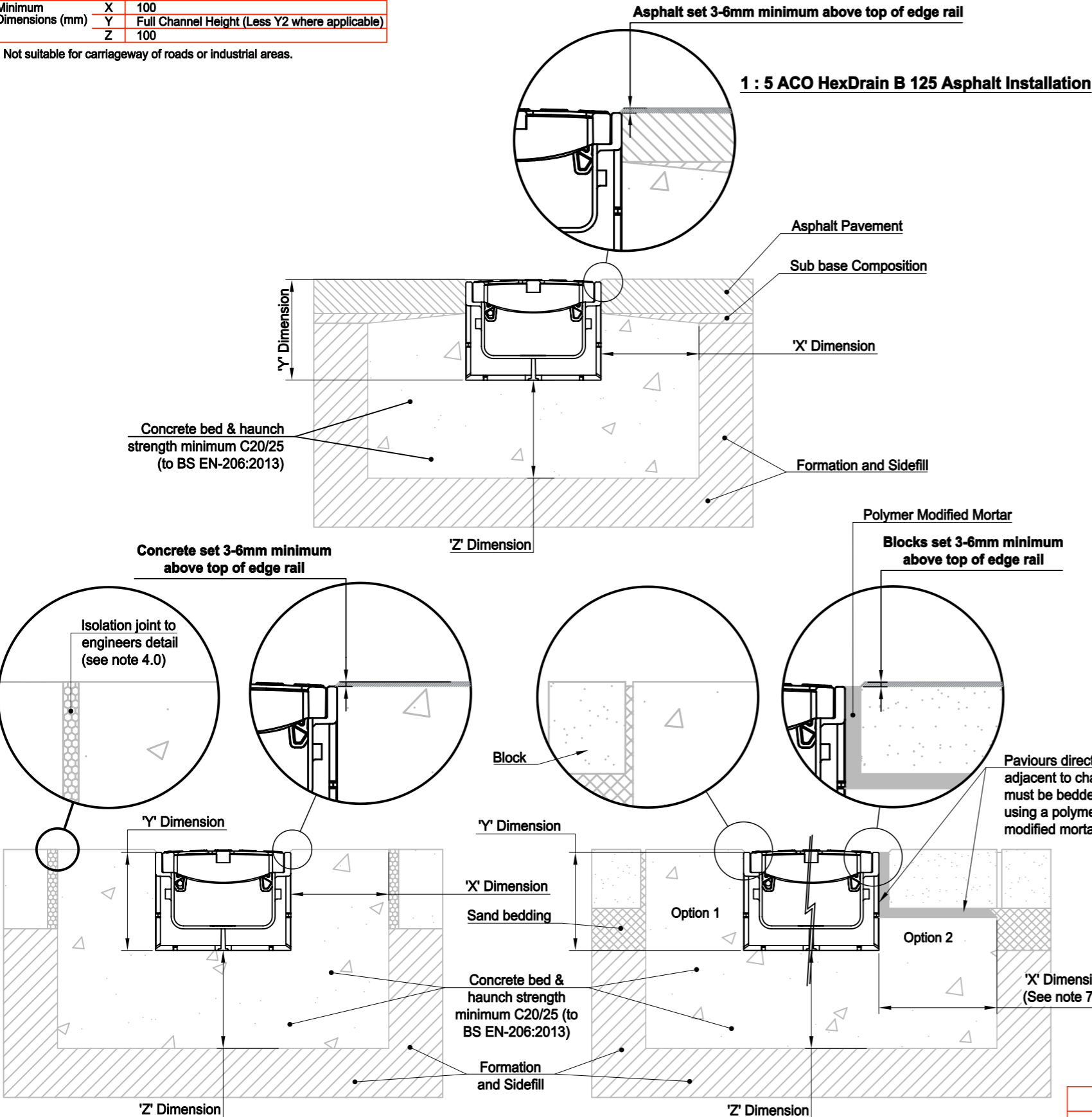
1 : 5 ACO HexDrain B 125 Concrete Installation
