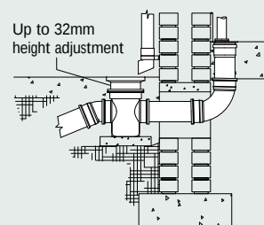
New Bottle Gully with Round Hopper
