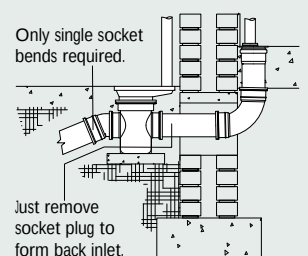
New Bottle Gully with Rectangular Hopper
