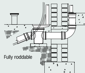
New Bottle Gully Rodding Access
