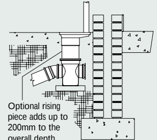
New Bottle Gully with Rectangular Hopper & Riser
