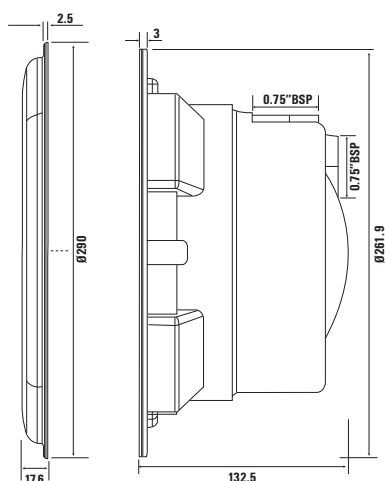
Niche & Fascia Ring
