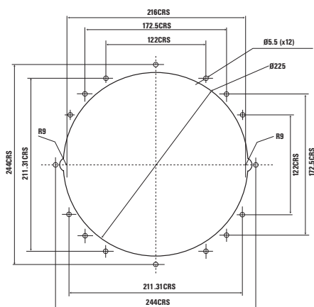
Panel Mount Cut Out Details
